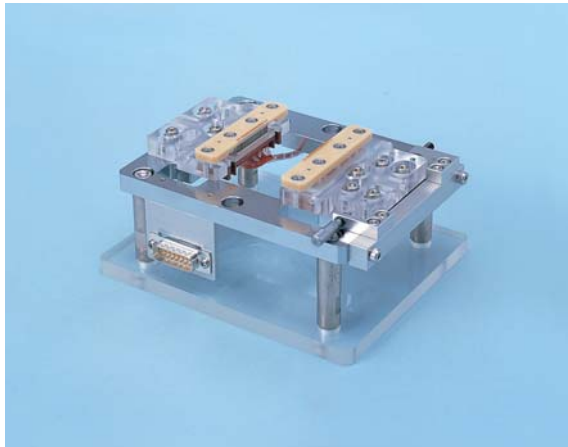
Small Sized Color STN Test Head
